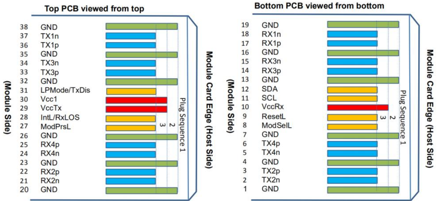
Figure 1 - QSFP112-compliant 38-pin connector
